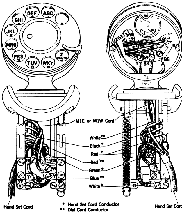
Fig. 10 - 214B, C, D Hand Telephone Sets
